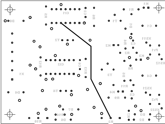
Bottom auxiliary 1 / Bottom insulated wire - Fata auxiliara jos 1 / Fire izolate fata de jos mirrored view - vedere in oglinda
